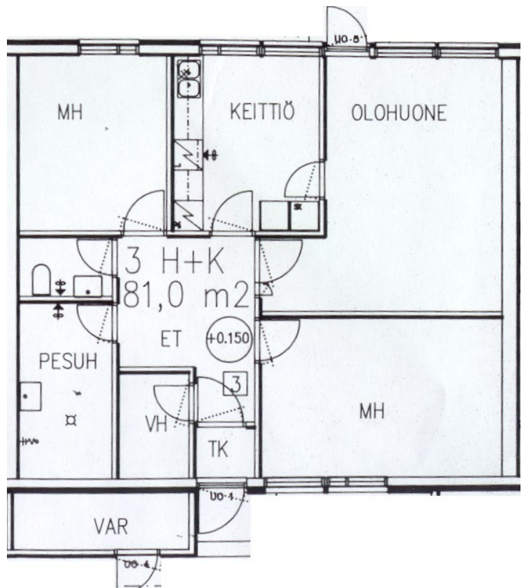
3h+k, 81,0 m 2
